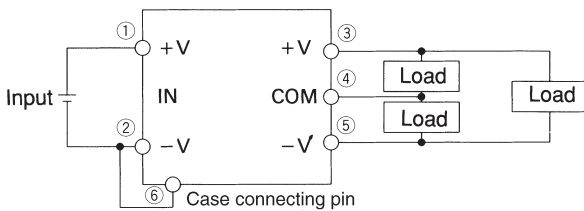
Fig.1.2 Dual output of pin connection
