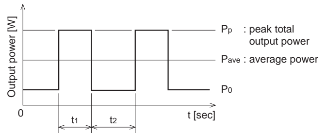
Fig. 4.11 Peak output power (ACE900F only)
