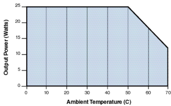
Maximum Output Power vs. Ambient Temperature
