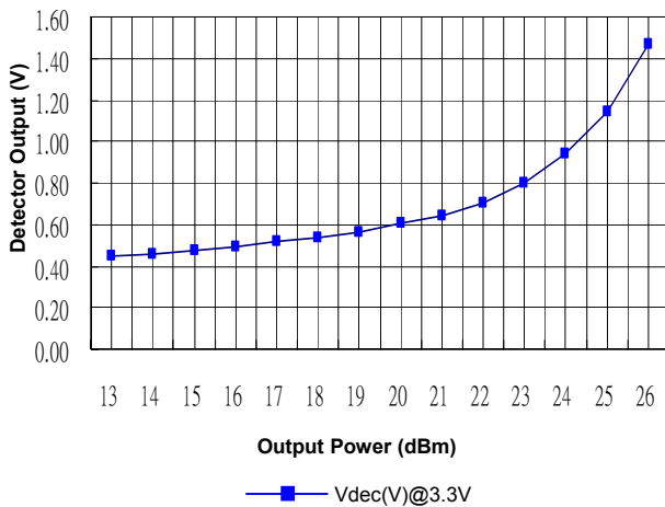
Detector Output vs. Output Power
