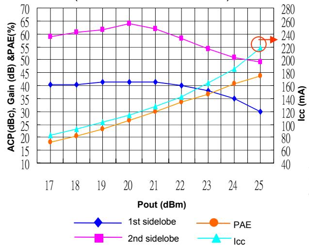
Gain, ACP, PAE, Icc vs Pout_3.3V (With 11b CCK Modulation)
