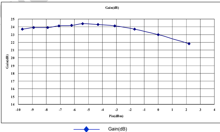
Power Gain vs. Pin
